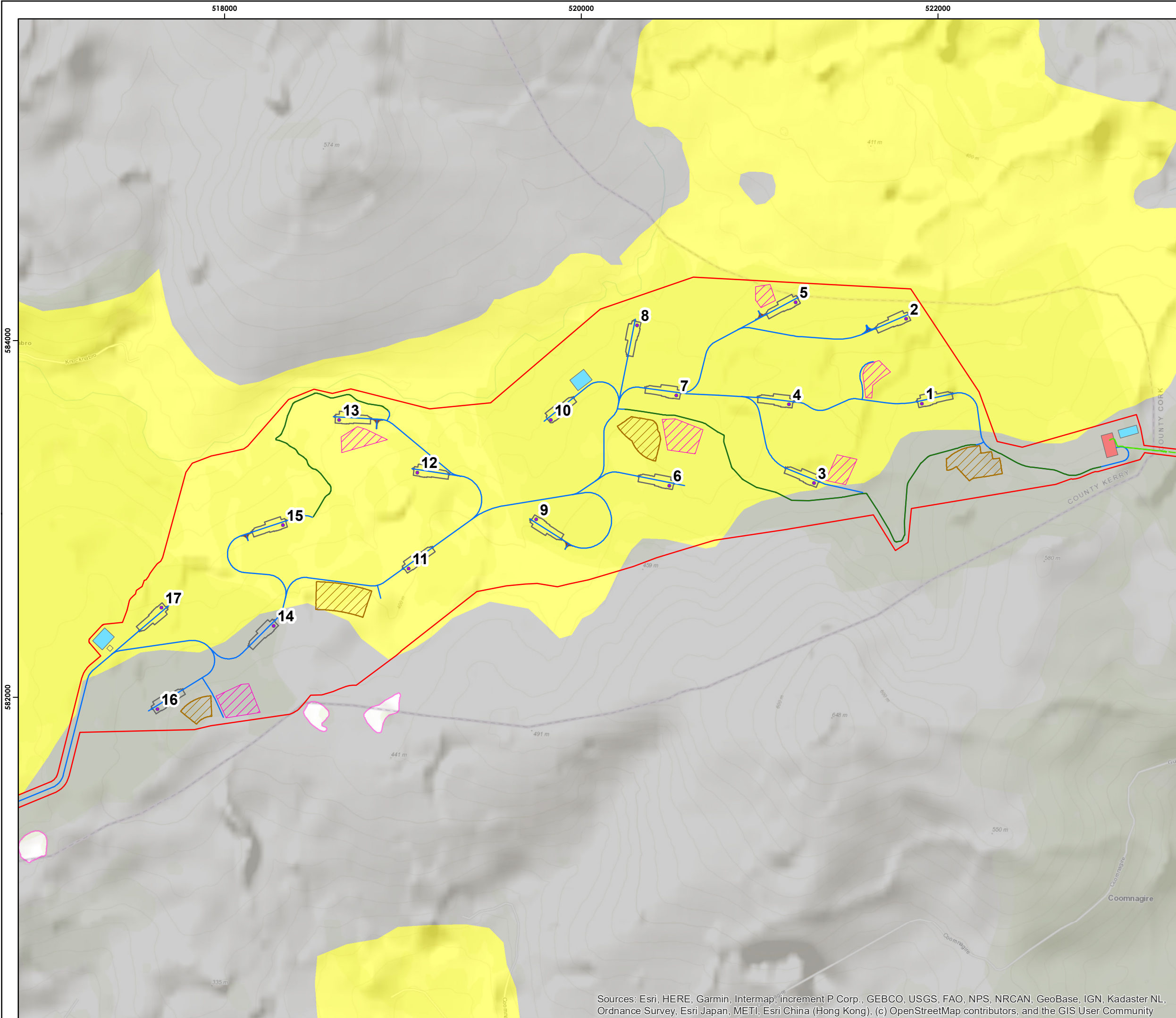
Figure10-6b Subsoil Permeability
